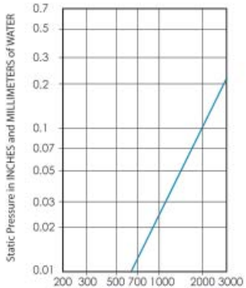
Pressure Drop - Damper Open (45" x 48")
