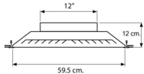
Fig.4 shows Section
