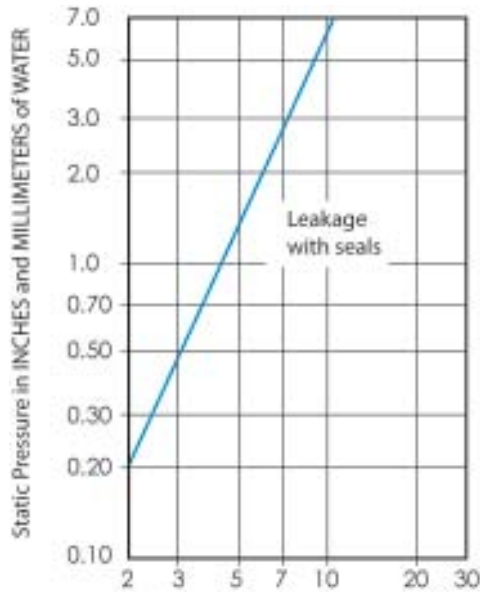
Air Leakage - Damper Closed (45" x 48")
