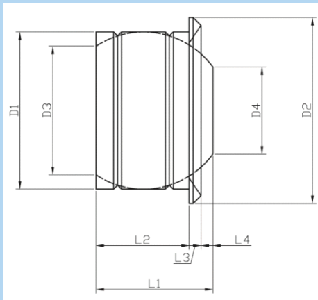
Fig.2 Section Detail
